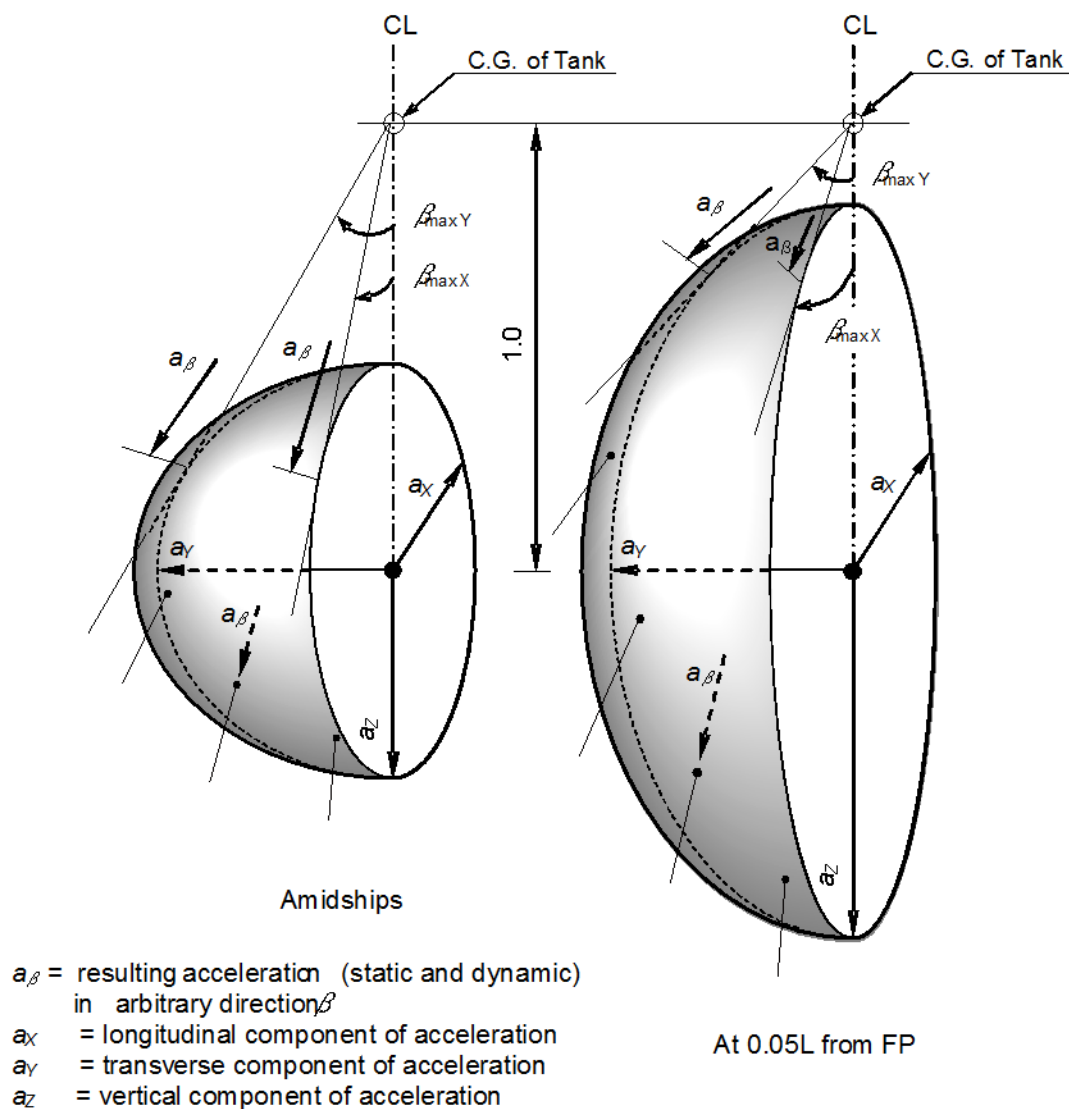
Figure 4.1 – Acceleration ellipsoid
